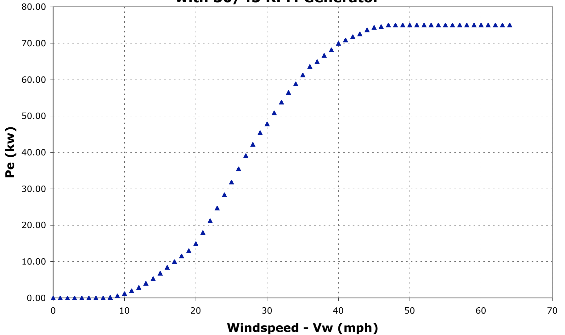
Figure 4. Windstar 1500 Power Curve for a 5 Turbine Array with 30/45 RPM Generator
